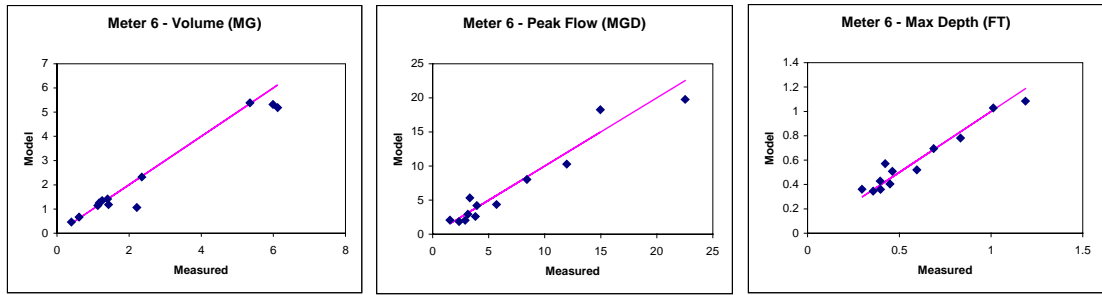
Figure 3-2. Example Calibration Event Scatterplots
