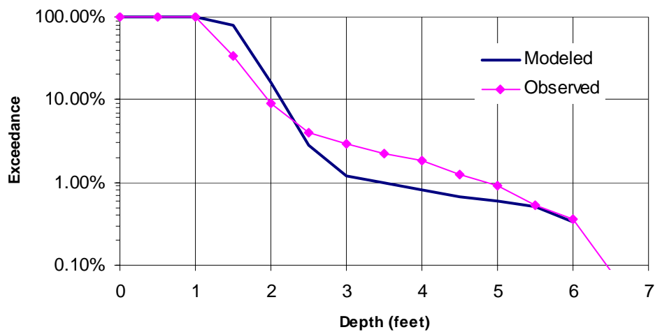
Figure 3-3. Example Long-term Depth Frequency Distribution Plot
