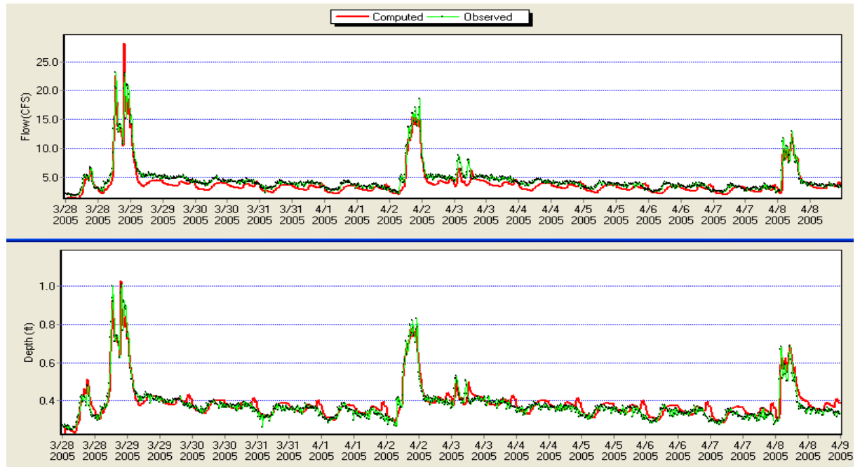
Figure 3-1. Example Time History Calibration Plots
