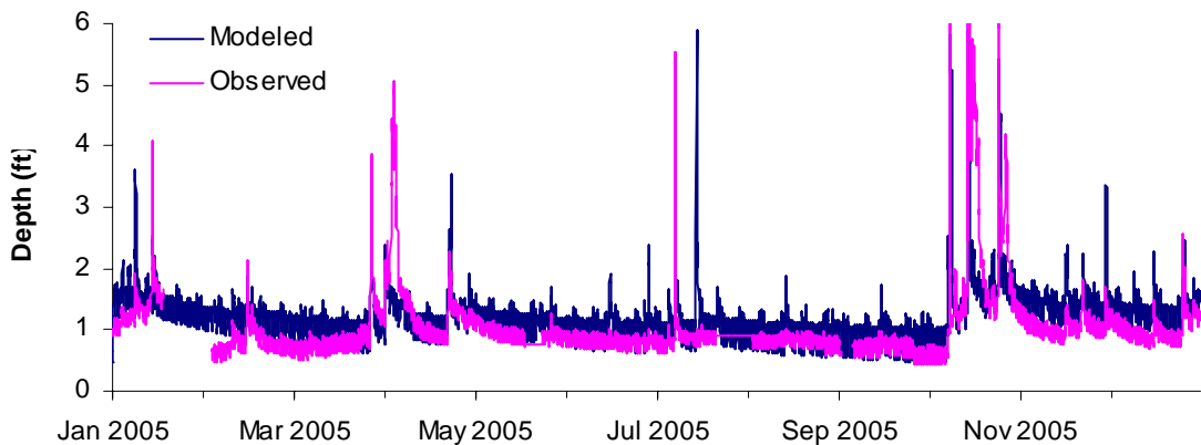
Figure 3-4. Example Long-term Depth Time Series Calibration Plot
